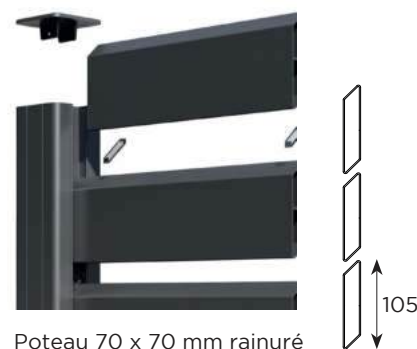
Poteau 70 x 70 mm rainuré
